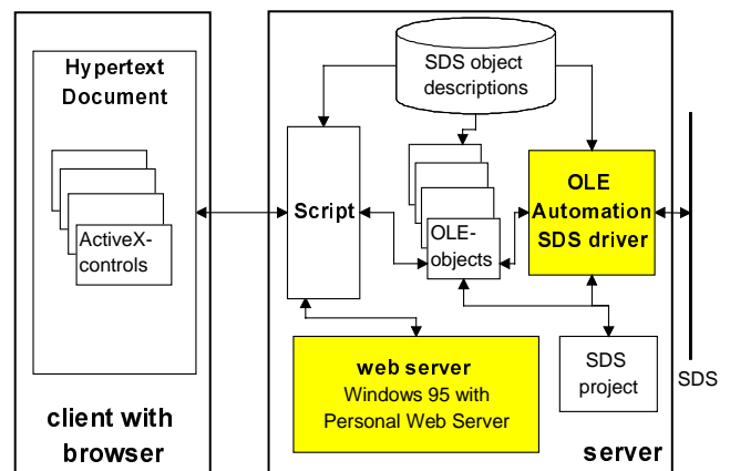
Figure 12. Topological structure of the SDS management implementation
