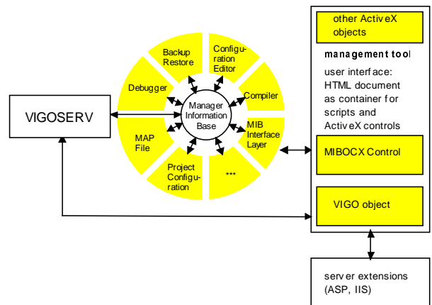
Figure 10. Relationship between the P-NET management tool and the MIB
