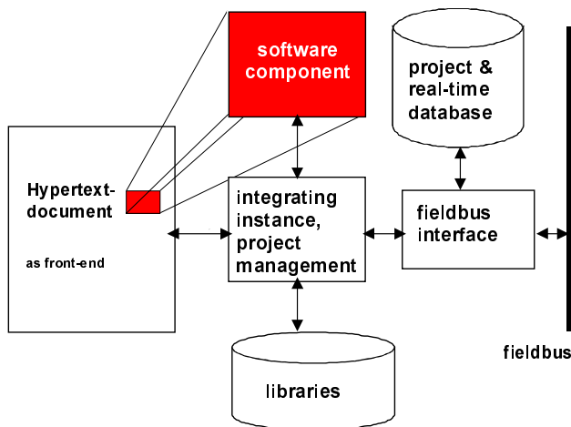
Figure 5. Structure of an Intranet based fieldbus management solution
