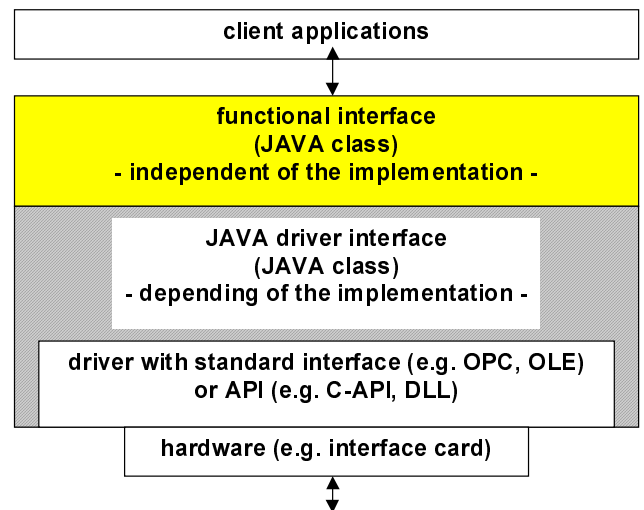
Figure 7. JAVA based data access
