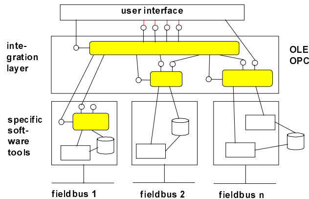
Figure 6. OLE/OPC as an integration layer for different fieldbusses
