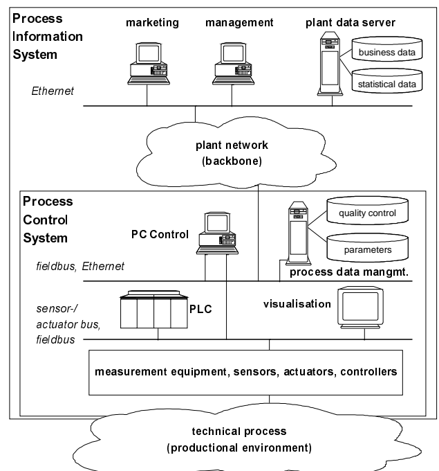
Figure 1. Process information system
