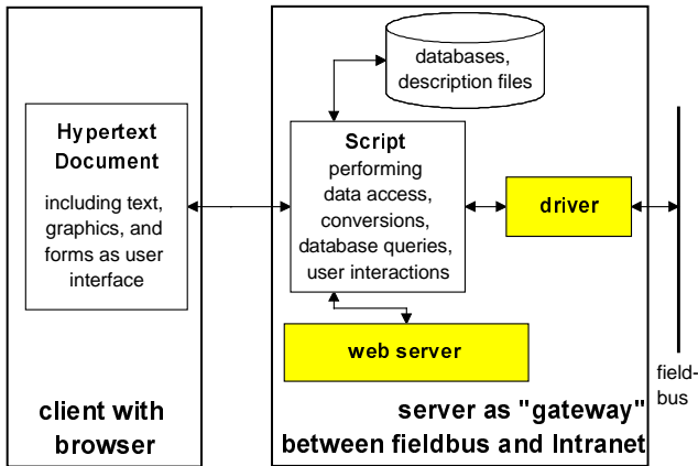
Figure 8. Data access from a hypertext document to a fieldbus
