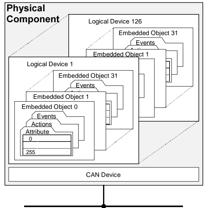
Figure 3. Embedded Objects in a SDS-device as function blocks
