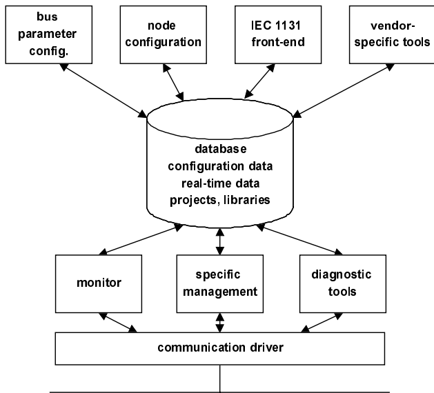
Figure 4. Principal structure of software tools for fieldbusses
