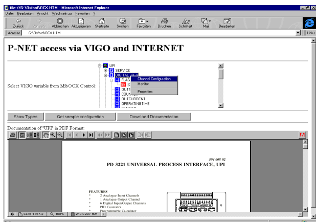
Figure 11. Screenshot of a compound document using ActiveX controls
